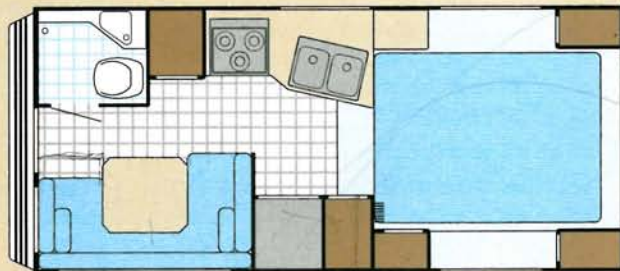
Lance 1010 – 10' 1" Popular floorplan with a large bath and a dinette capable of sleeping adults. Great length for convenience and excellent towing capabilities. New generator option.
