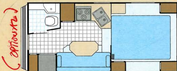
Lance 920 – 9' 6" This open floor plan features a roomy bath and front dinette with fold-over sofa and a view window. (Folding bunk bed with standard window is optional).
