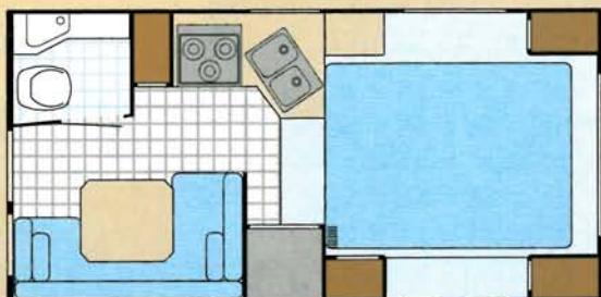
Lance 810 – 8' 6" Full galley, comfortable dinette, bathroom with shower, toilet, and split holding tank. Queen bed, ample storage and removable counter.
